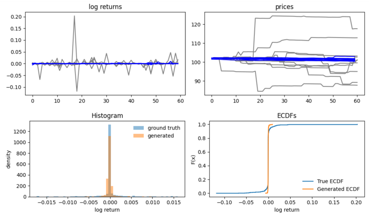
Figure 20: VG – GARCH
