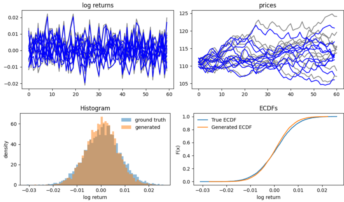
Figure 7: CEV – KRR
