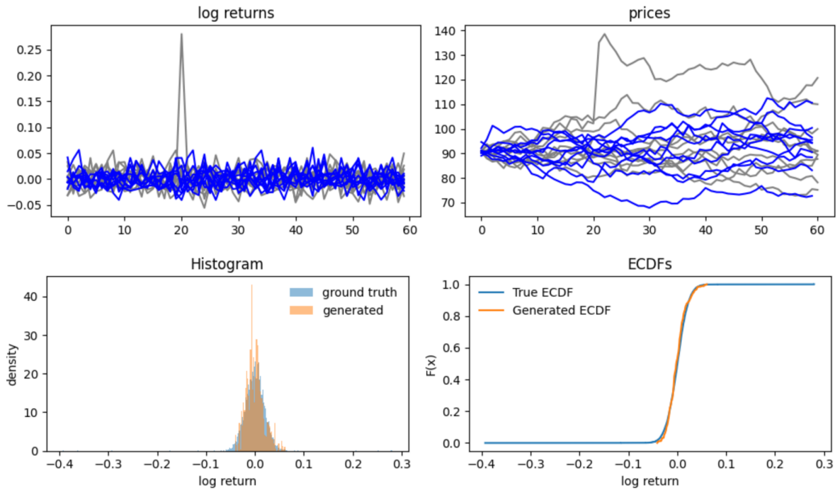
Figure 13: Merton – Hybrid KRR
