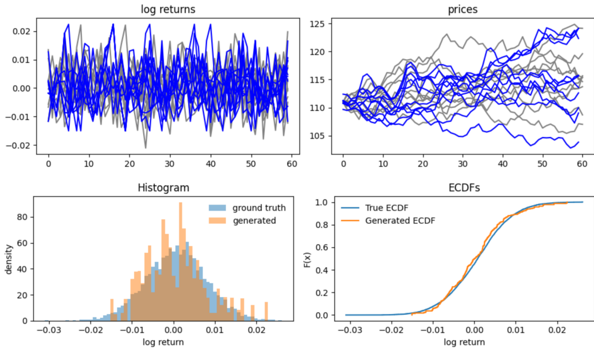
Figure 6: CEV – Bootstrap
