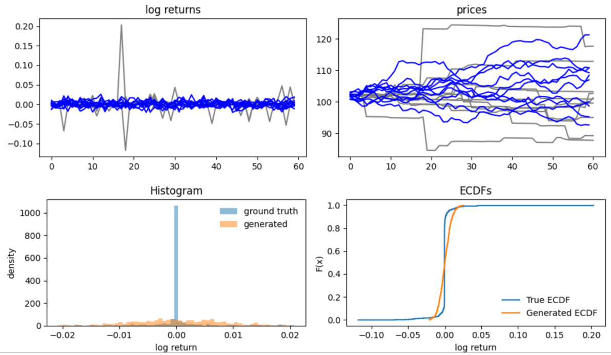
Figure 19: VG – ARIMA
