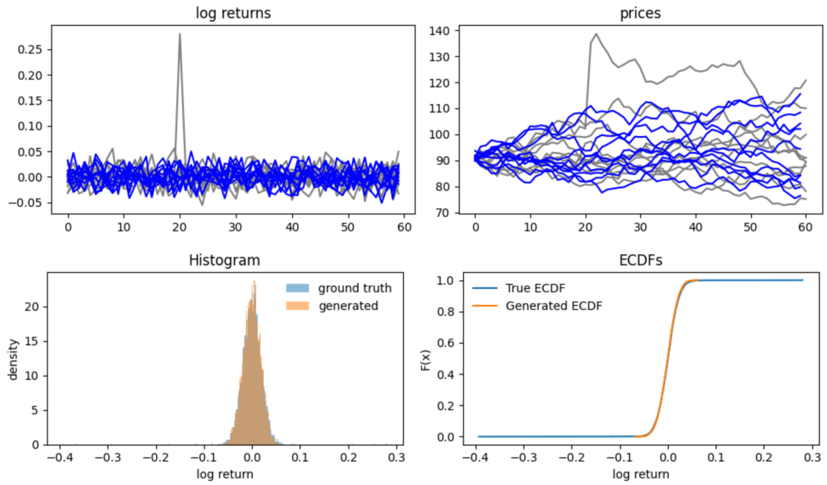
Figure 14: Merton – ARIMA
